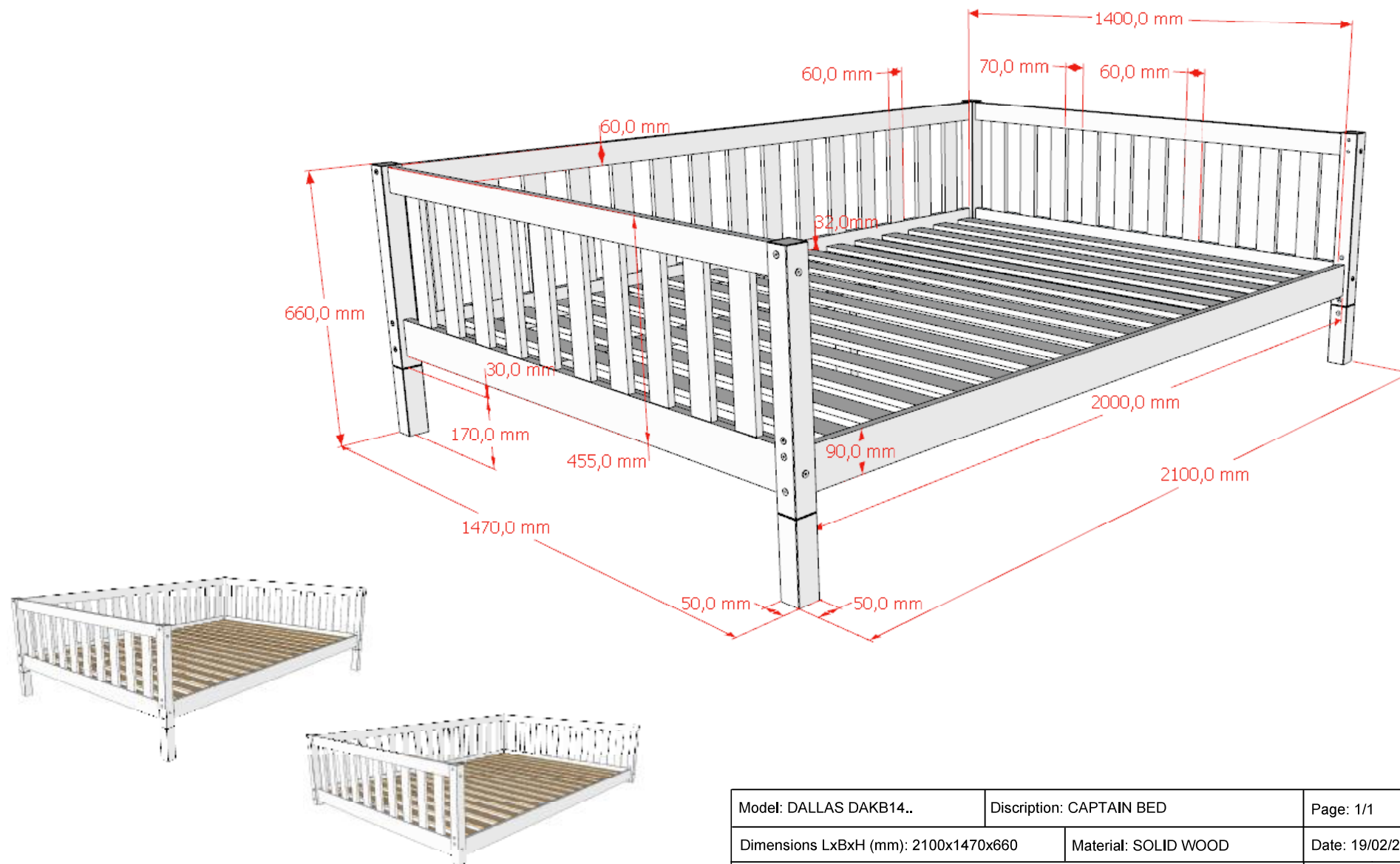
CAPTAIN BED WITH REMOVABLE LEGS TO MAKE A FLOORBED
