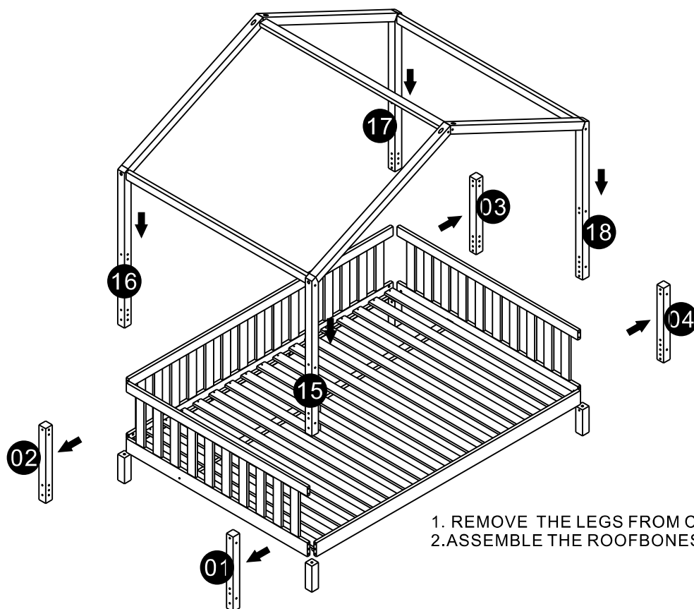
CAPTAIN BED DAKB140..+ ROOF DARF140..
